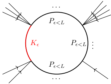
Fig. 1. The second term in Equation (24) representing the holomorphic anomaly
